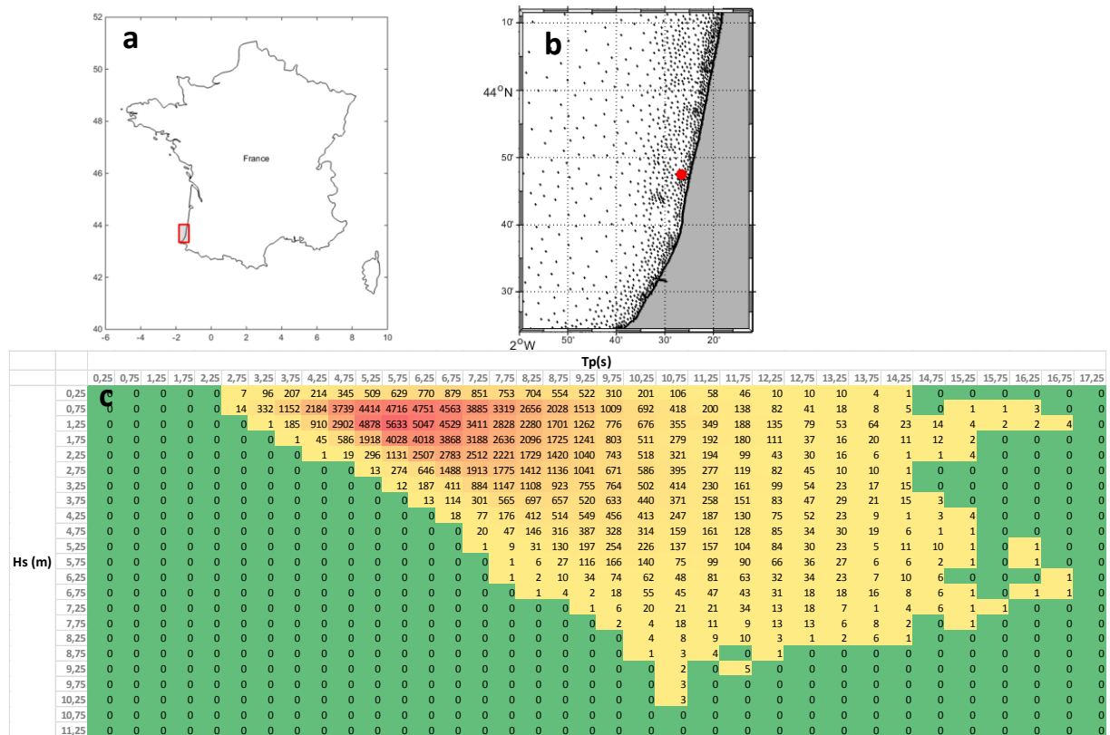
Figure: Example of ( H_s, T_p ) annual wave scatter diagram (c) at a specific geographic position (a and b, red dot) using data available from (here). This table was established based on 166560 ( H_s, T_p ) pairs, delivered by Homere hindcast (Bouidière et al. 2013). Scatter diagrams are available from here at all points of the hindcast mesh (b, black dots). The study area covers the entire west coast of France.
